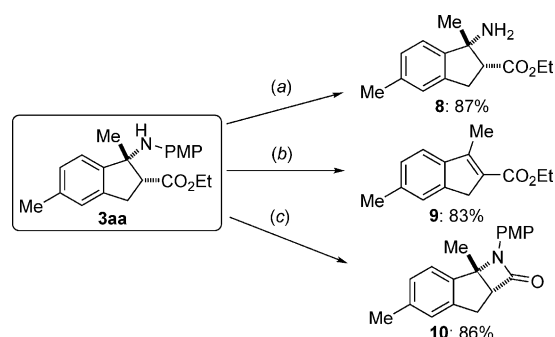
Scheme 7. Diversification of product 3aa . Reagents and conditions: a) CAN (2.5 equiv), \text{CH}_3\text{CN}/\text{H}_2\text{O} (1:1), 23 °C, 3 h. b) Toluene, 160 °C, 14 h. c) LiHMDS (1.5 equiv), THF, 0 °C \rightarrow 23 °C, 10 h. CAN = ceric ammonium nitrate, LiHMDS = lithium bis(trimethylsilyl)amide.
